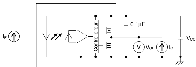
Test circuit for V_{OL}
